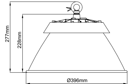
Tall Reflector
