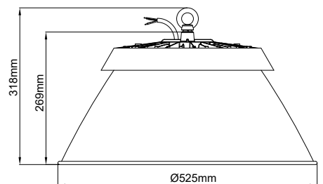
Tall Reflector
